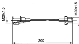
硬管接管 [YL]
